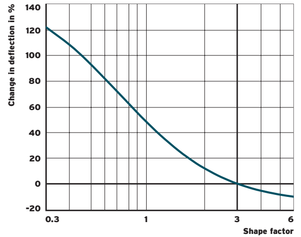
Fig. 6: Deflection 4 at constant thickness in relation to the shape factor
