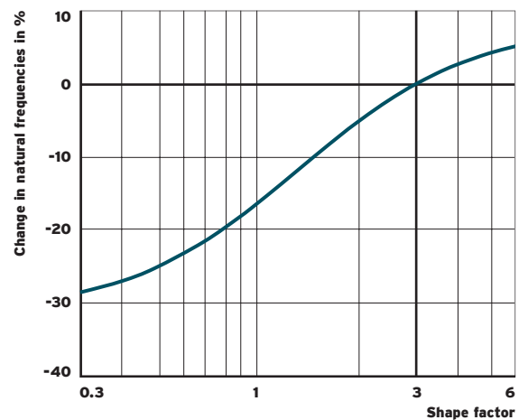
Fig. 8: Natural frequency 4 at constant thickness in relation to the shape factor
