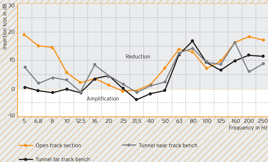
Effect of sleeper padding
