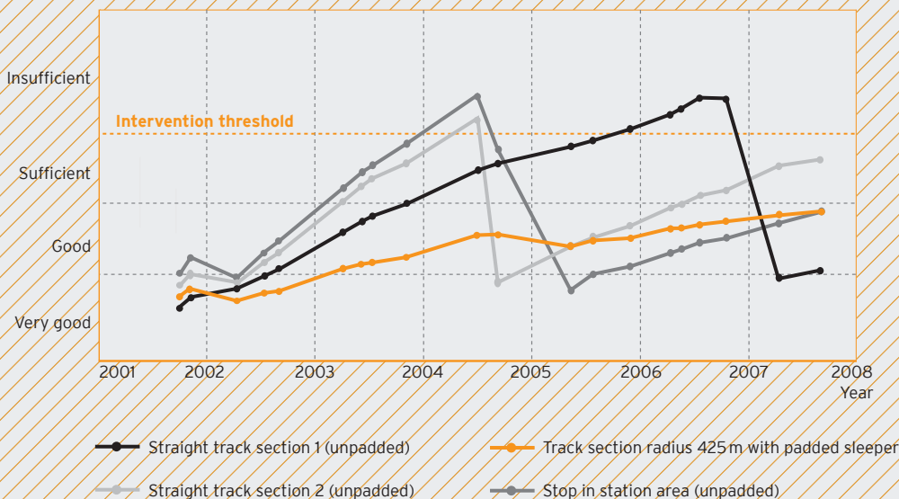
Track geometry quality
