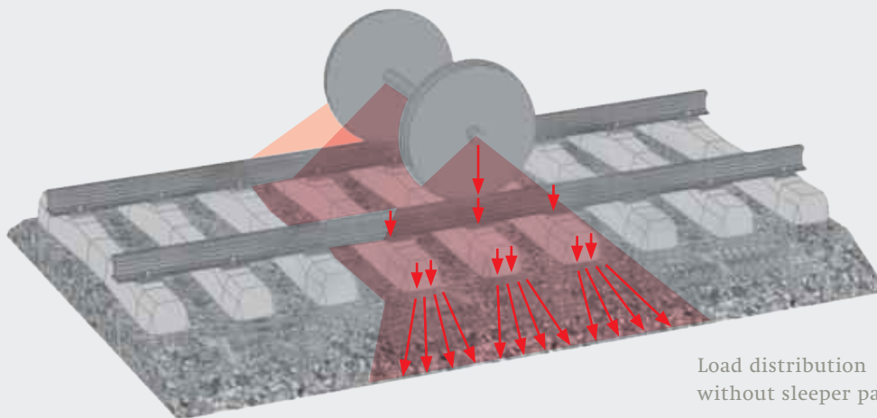
Load distribution with sleeper pads
