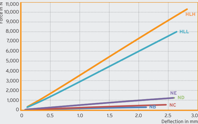
Isotop DZE-1
