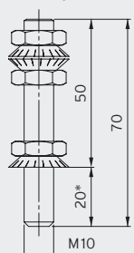
Isotop NV 1-9
