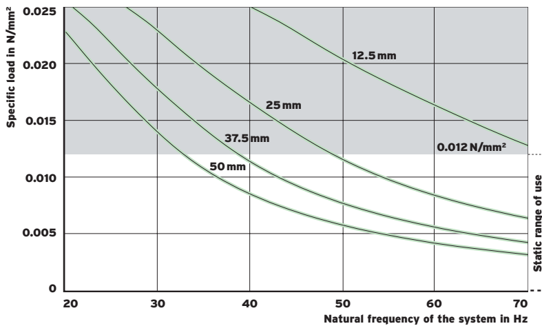
Fig. 3: Natural frequencies for different bearing thicknesses
