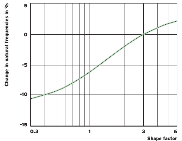
Fig. 8: Natural frequency 5 at constant thickness in relation to the shape factor
