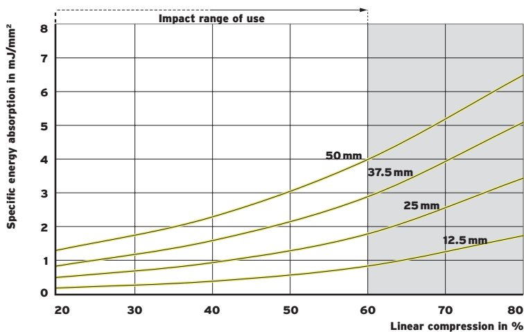
Fig. 4: Specific energy absorption for different bearing thicknesses
