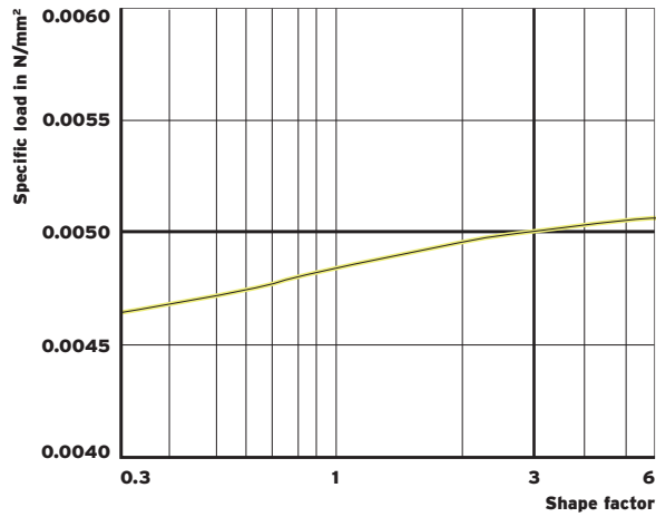
Fig. 5: Static range of use in relation to the shape factor
