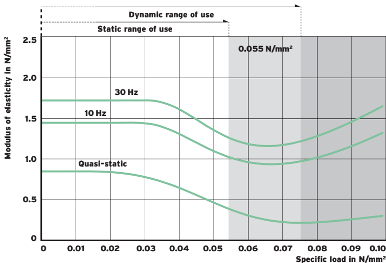
Fig. 2: Load dependency of the static and dynamic modulus of elasticity
