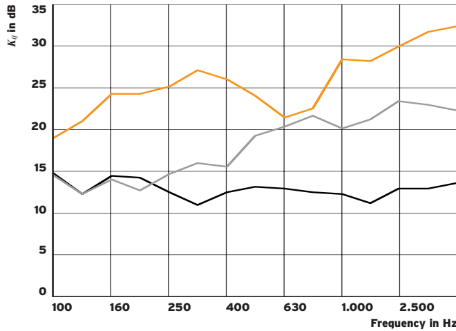
Abb. 2: K_{12} Plot for a T-joint with Syldyn® and elastic fastener, Syldyn® with rigid fastener and without elastomer intermediate layer
